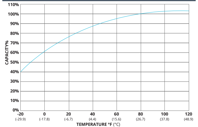
TEMPERATURE vs CAPACITY
